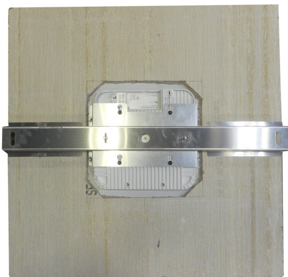
Back –Wide bracket distributes the weight of the access point to reduce strain on the ceiling tile.
