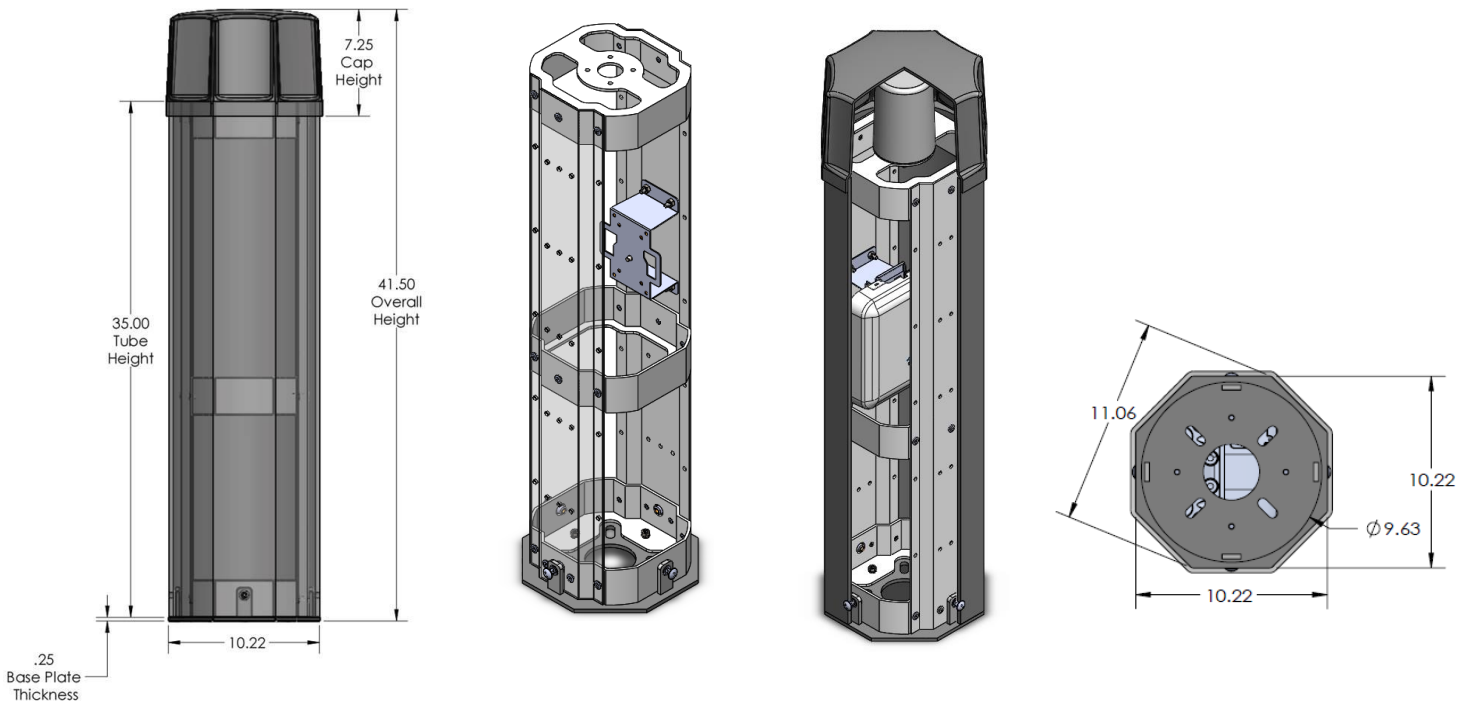
Octagonal Cap Bollard
