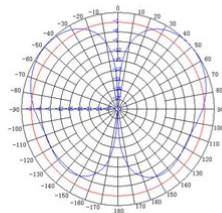
Vertical Radiation at 5 GHz
