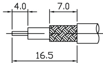
STRIPPING DIMENSION
