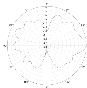
E-Plane Pattern
