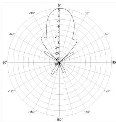
E-Plane Pattern
