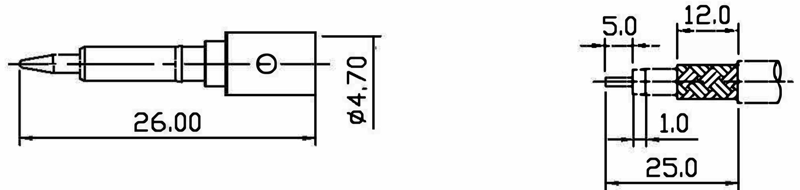
STRIPPING DIMENSION
