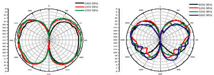
V-plane Co-polarization Pattern
