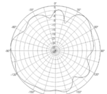
H Plane
