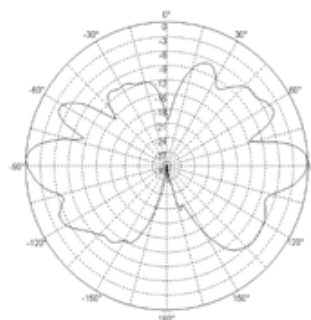
E Plane
