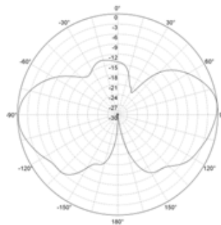
E Plane
