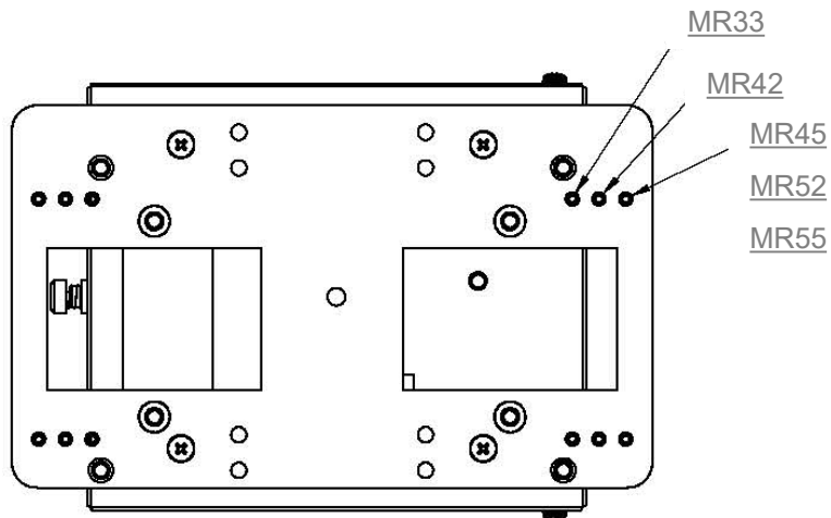
Adapter Plate for Aruba APs SKU: 231728
