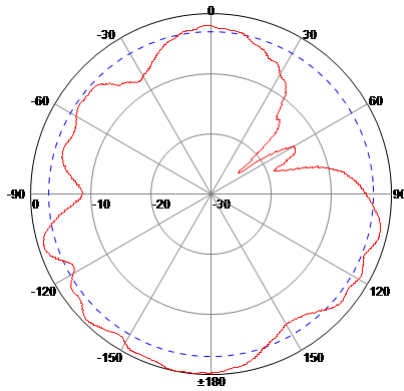
H Plane
