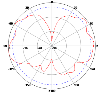
E Plane
