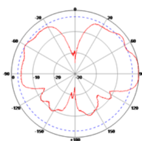
E Plane
