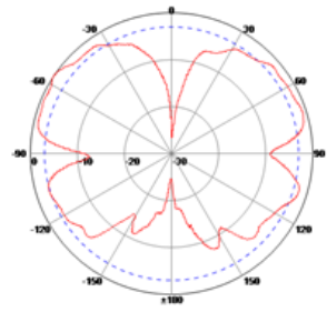
E Plane
