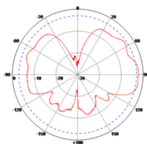
E Plane
