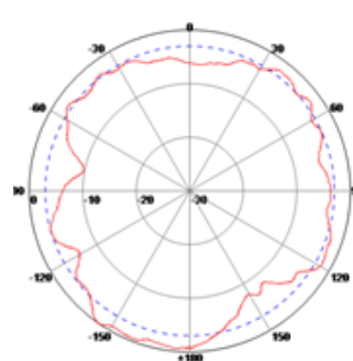
H Plane
