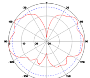
E Plane
