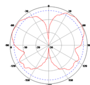
E Plane
