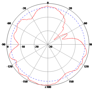
Port 4: 5 GHz
