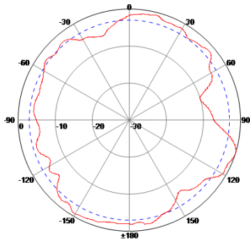
Port 2: 5 GHz
