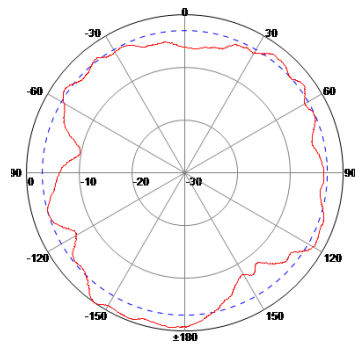
H Plane
