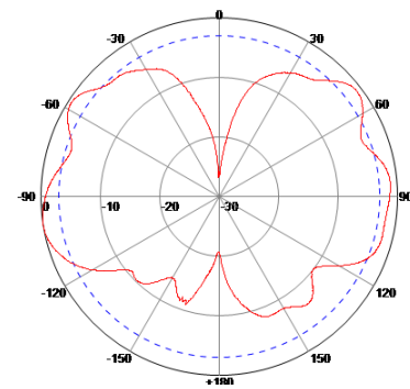
E Plane
