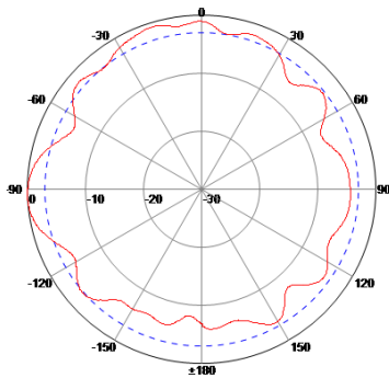
Port 4: 2.4 GHz
