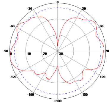
E Plane
