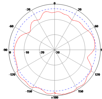
Port 3: 2.4 GHz
