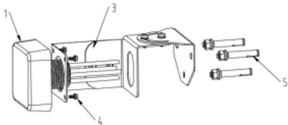
Installation Sketch
