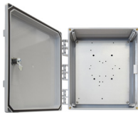
14x12x6 Polycarb Solid Door, Key Lock 4 N-Style Holes Tessco No 516093
