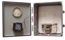
14x12x6 Heated/Cooled Solid Door, Latch Lock No Holes Tessco No 538828
