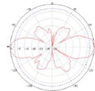
5 GHz E Plane
