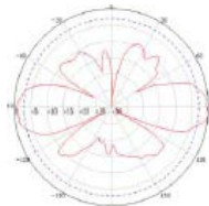
6 GHz E Plane
