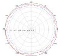
6 GHz H Plane
