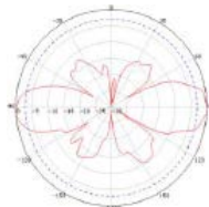
5 GHz E Plane
