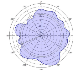
5.1-5.9 GHz H Plane
