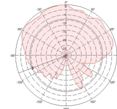
5.1-5.9 GHz E Plane
