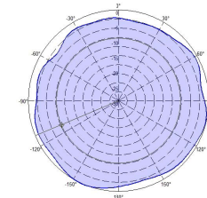
2.4-2.5 GHz H Plane
