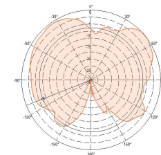
2.4-2.5 GHz E Plane
