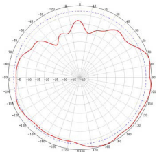
Port 2 2.4 GHz E Plane
