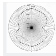
H Plane
