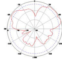
Port 1 5 GHz E Plane
