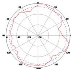
Port 2 5 GHz H Plane
