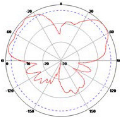
Port 2 5 GHz E Plane
