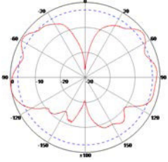
Port 1 2.4 GHz E Plane
