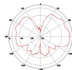
Port 3 2.4 GHz E Plane
