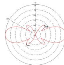
5/6 GHz E Plane
