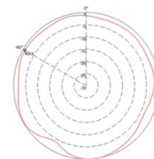
5/6 GHz H Plane
