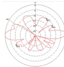
2.4 GHz E Plane
